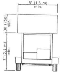
TYPE B ROOF OR TRAILER MOUNTED
