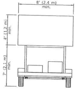
TYPE C TRAILER MOUNTED
