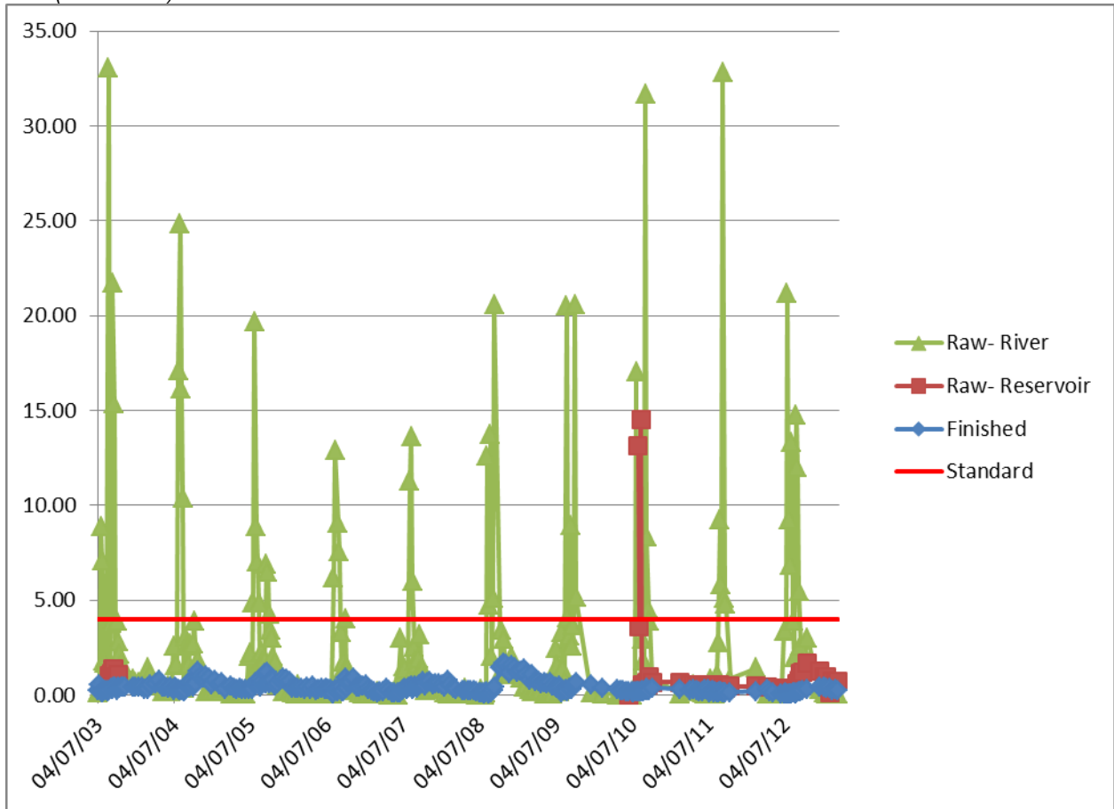
Figure 5. Atrazine Data from Syngenta for Wayne City Side Channel Reservoir (Raw and Finished Water) and Skillet Fork (Raw Water)
