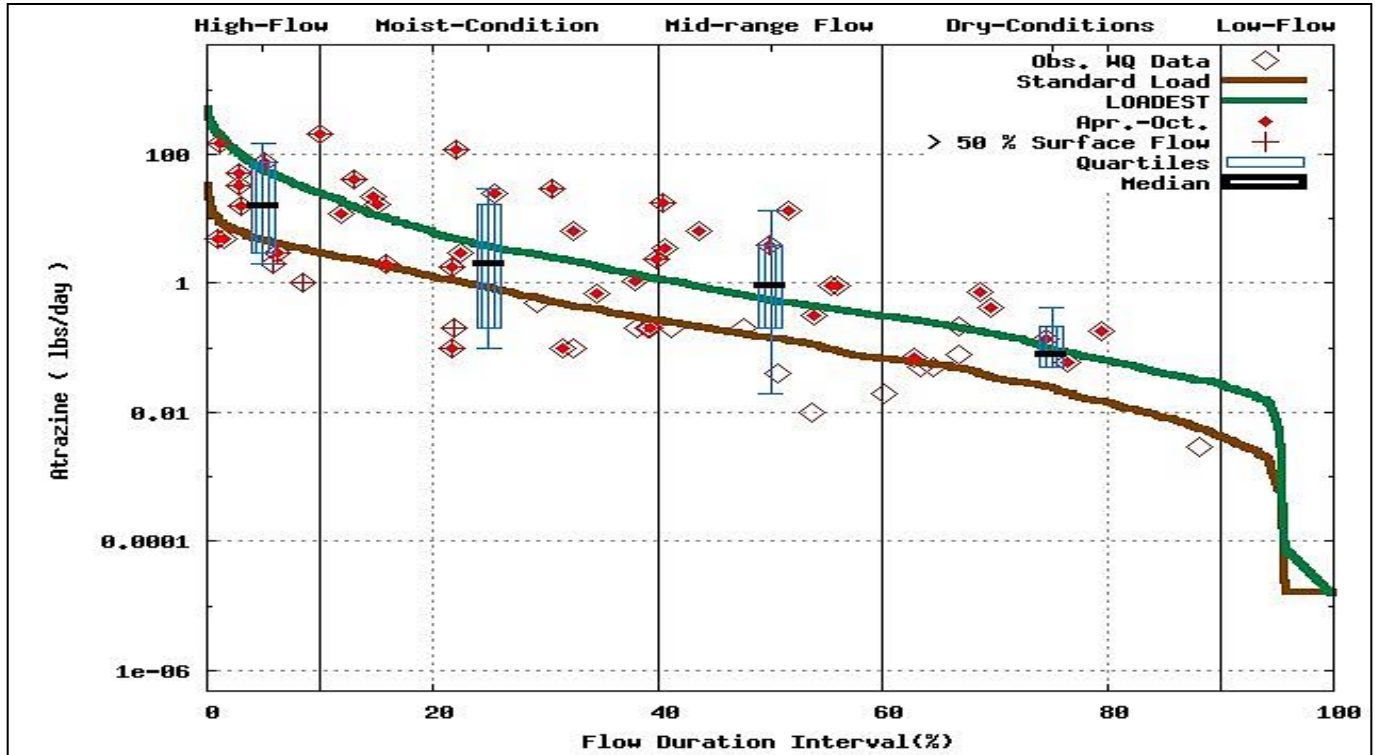
Figure 6. Load Duration Curve from Illinois EPA derived using flow data from USGS stream gage 03380500 and Syngenta provided data set for atrazine loadings to Skillet Fork .
