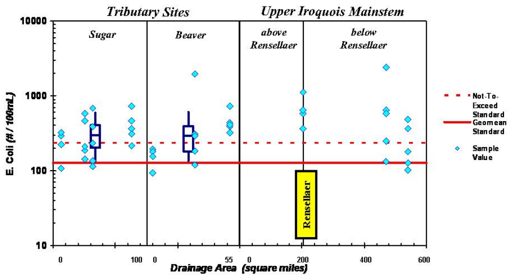
Figure 38. Lower Iroquois Tributary versus Upper Iroquois Mainstem Drainage Area Profile
