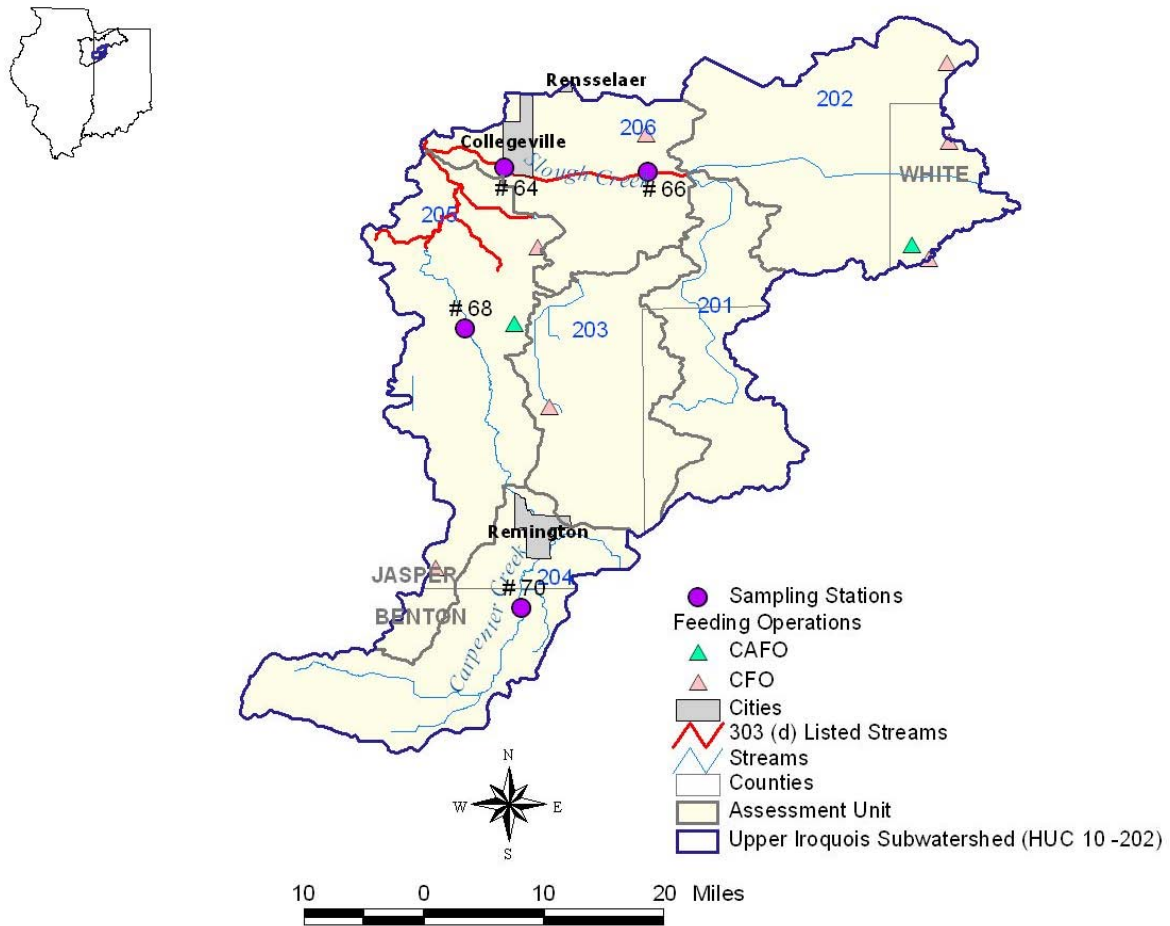
Figure 88. Feeding Operations in the Slough Creek Subwatershed (HUC10-202)
