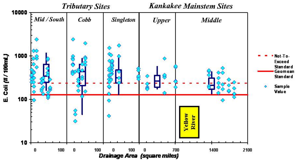
Figure 31. Middle Kankakee Tributary versus Mainstem Drainage Area Profile
