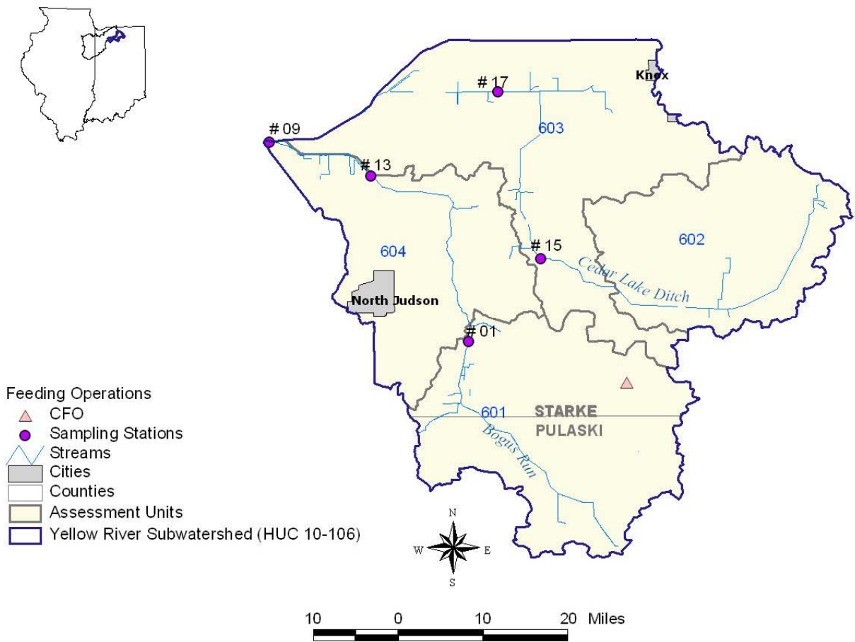
Figure 83. Feeding Operations in the Kline Arm Subwatershed (HUC10-106)
