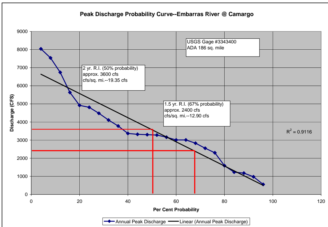
Figure 4. Annual Peak Discharge Probability Curve @ Camargo 1981-2004
