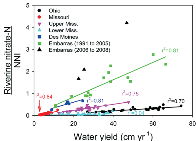
Fig. 3. Annual riverine nitrate N loads divided by net N inputs (NNI; average of previous 4 yr) plotted against annual water yield of the river for the major Mississippi River subbasins (1979–2007), as well as the Des Moines River in central Iowa (2001–2006) and Embarras River in east-central Illinois (1991–2008).
