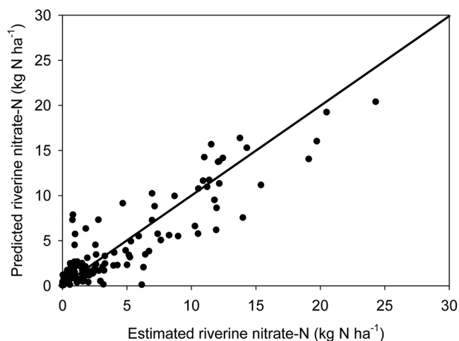
Fig. 7. Predicted riverine nitrate N yields, January to June, for 153 unique subwatersheds in the Mississippi River basin for 1997 to 2006 compared with estimated yields from measurement data.
