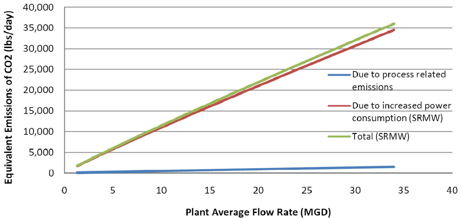
Figure 10: Estimated Increase in Emissions in SRMW Subregion (Direct and Indirect)
