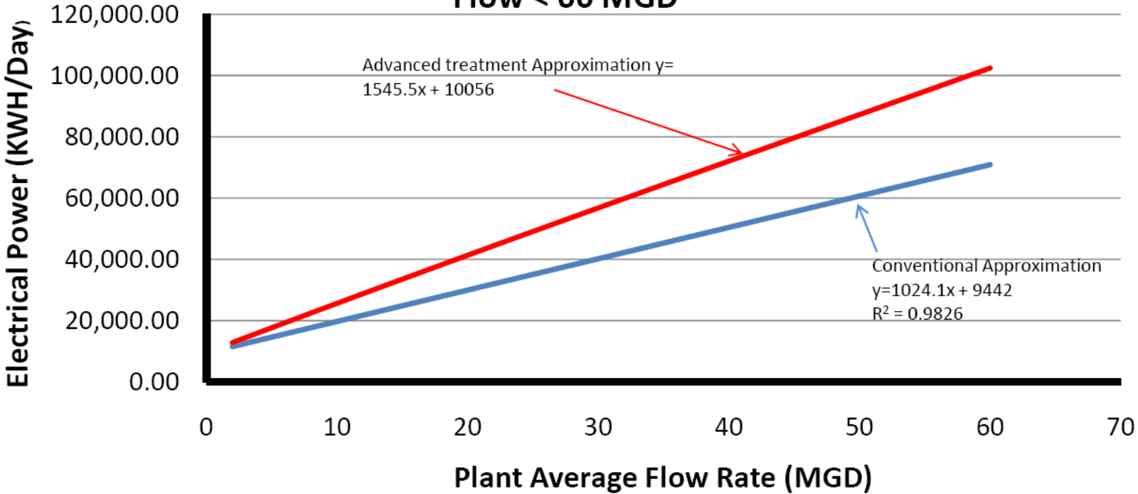
Figure 6: IAWA Power Estimates Conventional vs. Advanced Flow < 60 MGD
