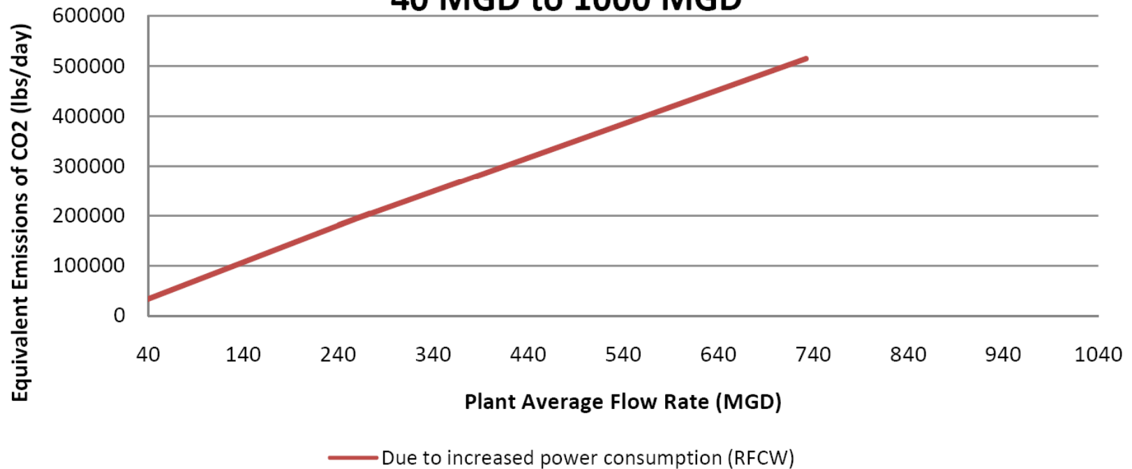
Figure 7A: Estimated Increase in Indirect Emissions in RFCW Subregion for Plant Flows from 40 MGD to 1000 MGD
