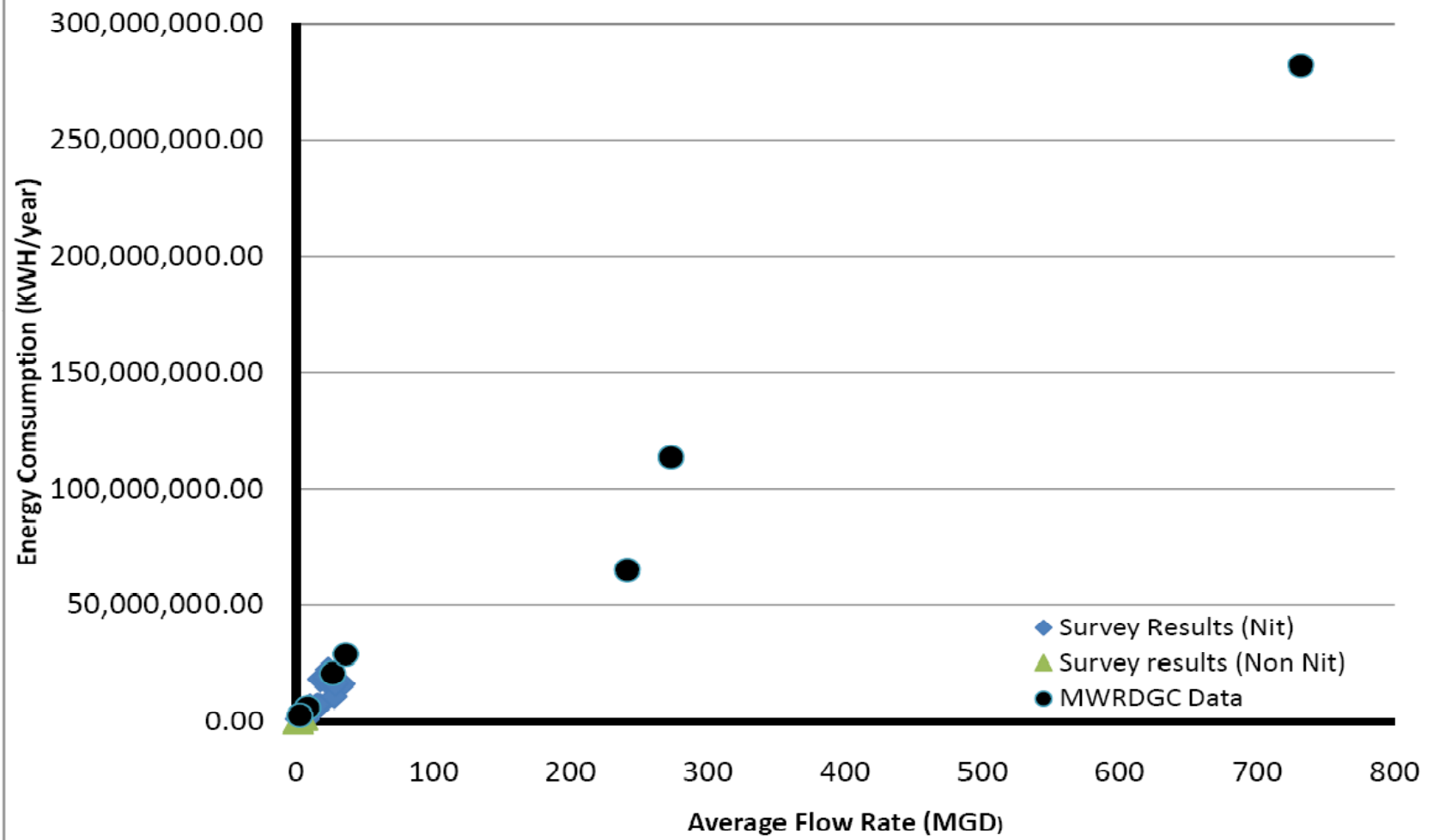
Figure 5A: Energy Consumption from Survey Results for Non-Nitrifying and Nitrifying Treatment Plants, All Flows
