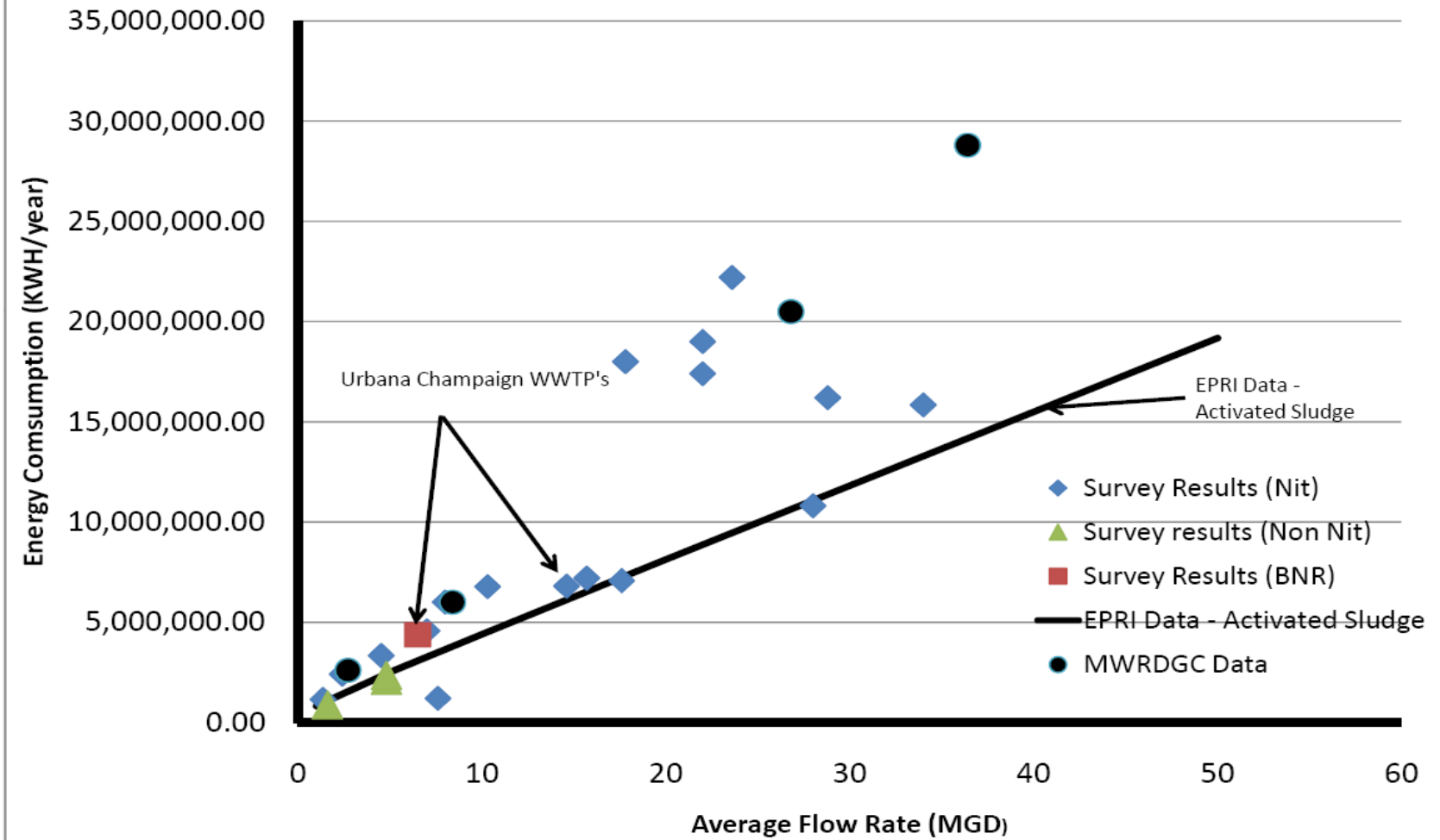
Figure 5: Energy Consumption from Survey Results for Non-Nitrifying and Nitrifying Treatment Plants with Flow < 40 MGD
