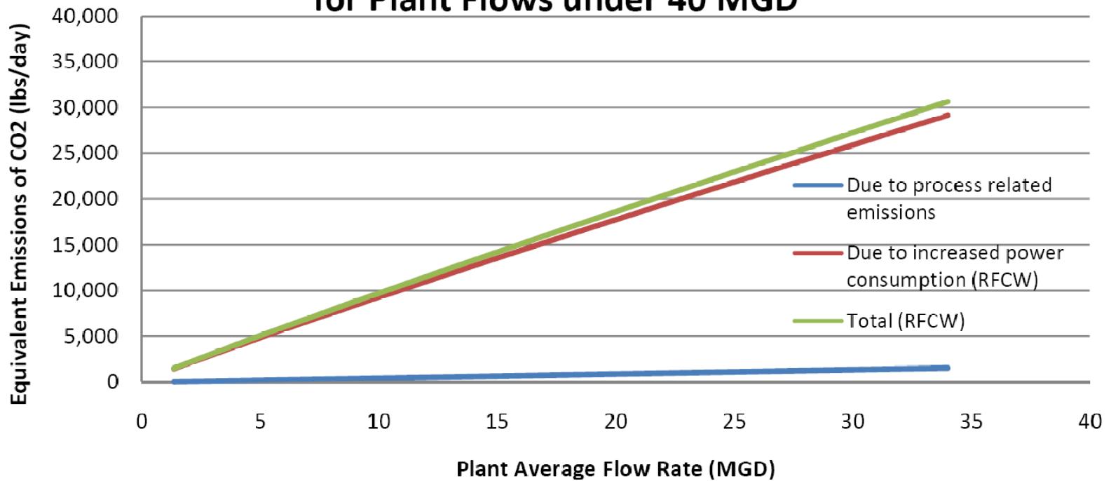
Figure 9: Estimated Increase in Emissions in RFCW Subregion (Direct and Indirect) for Plant Flows under 40 MGD
