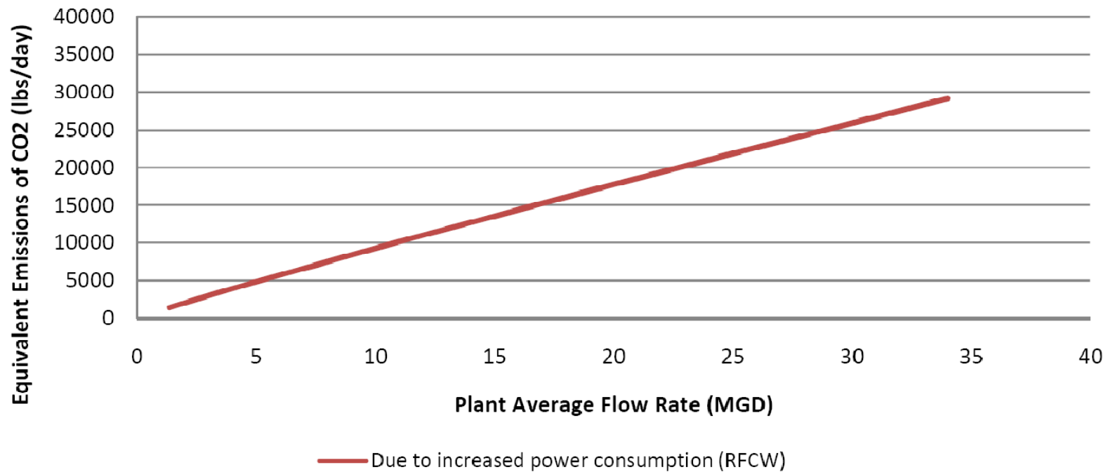
Figure 7: Estimated Increase in Indirect Emissions in RFCW Subregion for Plant Flows under 40 MGD
