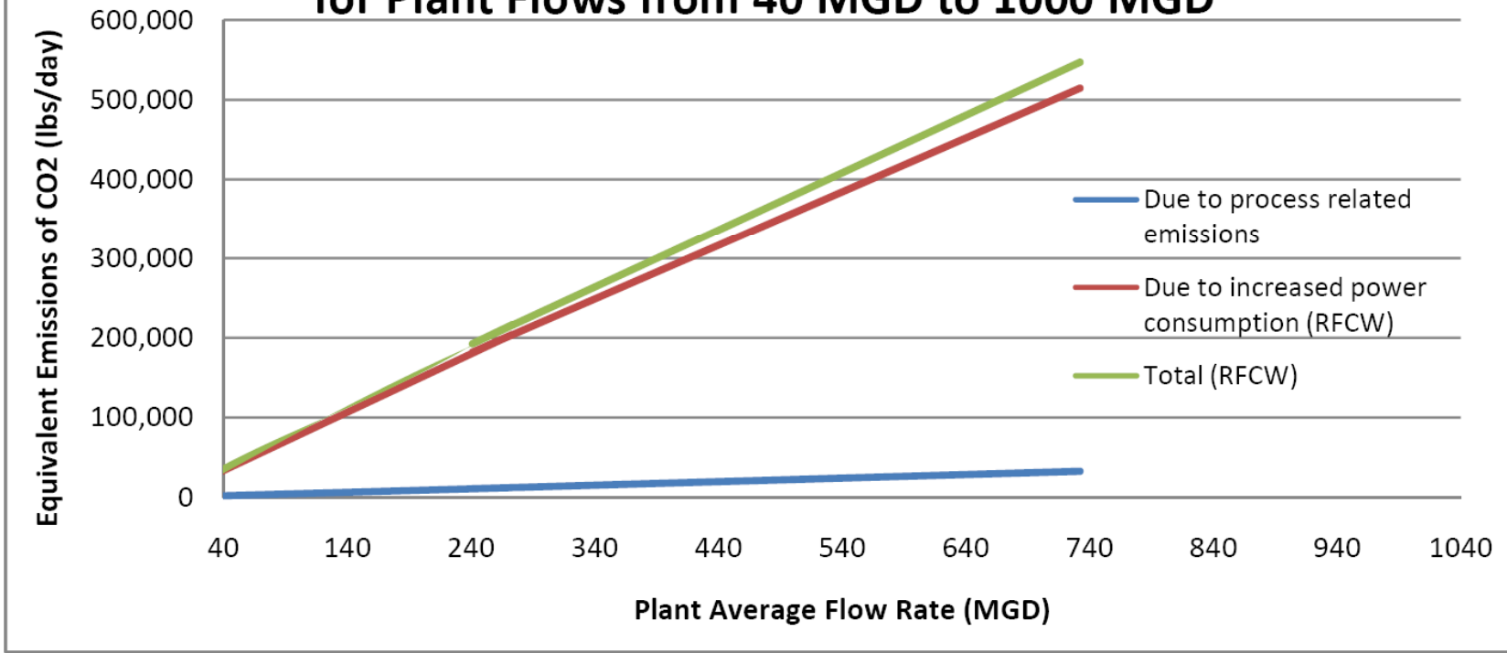
Figure 9A: Estimated Increase in Emissions in RFCW Subregion (Direct and Indirect) for Plant Flows from 40 MGD to 1000 MGD
