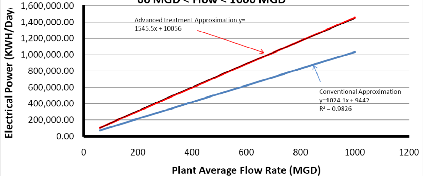
Figure 6A: IAWA Power Estimates Conventional vs. Advanced 60 MGD < Flow < 1000 MGD
