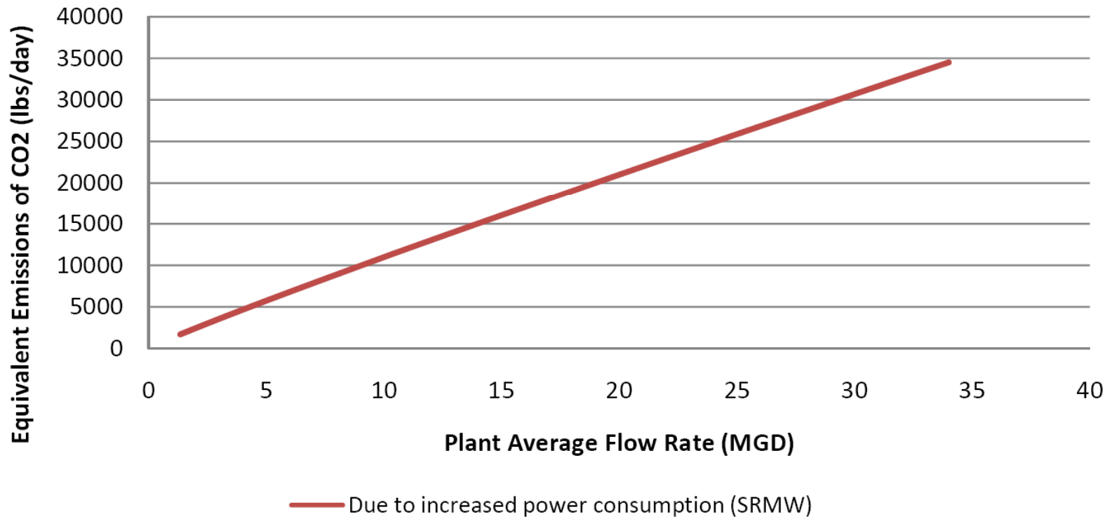
Figure 8: Estimated Increase in Indirect Emissions in SRMW Subregion
