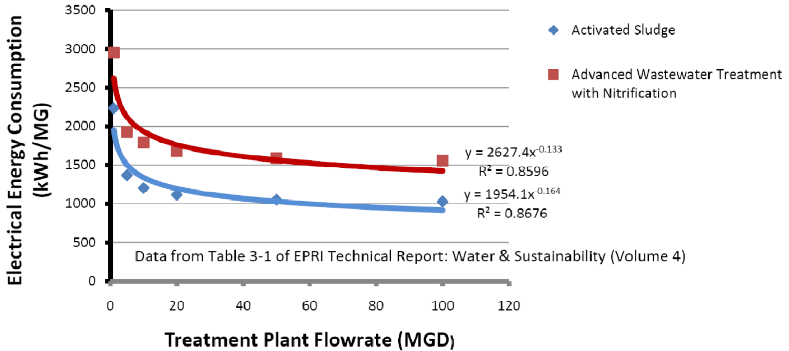
Figure 4: Electricity Consumption vs. Plant flow rate
