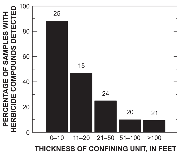
Figure 14. Relation of frequency of detection of herbicides and their transformation products in source-water aquifers in Illinois to thickness of the confining unit, 2001-02 (>, greater than; total number of samples in classification is shown above bar, confining-unit thicknesses were not available for 12 sampled wells).
