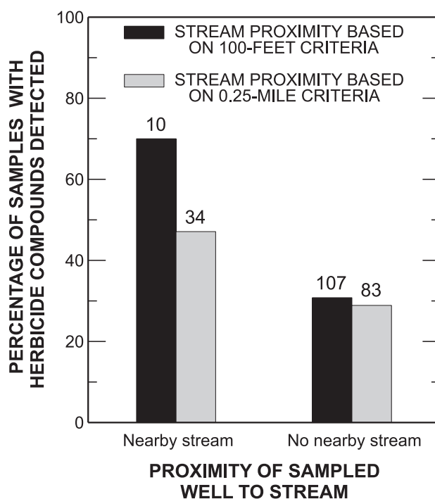
Figure 17. Relation of frequency of detection of herbicides and their transformation products in source-water aquifers in Illinois to proximity of well to a stream, 2001-02 (total number of samples in stream-proximity interval is shown above bar)
