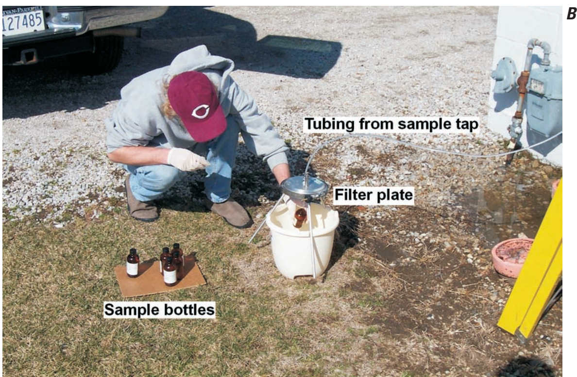
Figure 5. Ground-water sampling at well 47725, Oreana, Ill., for analysis of herbicide compounds: (A) routing of discharge from the well through Teflon tubing to a 0.7-micron, baked, glass-fiber filter enclosed in a stainless-steel filter plate, and (B) collection of samples in 125-milliliter, amber, baked-glass bottles (refer to figure 3, Macon Co., for well location; photographs by Steven E. Stammer, U.S. Geological Survey).
