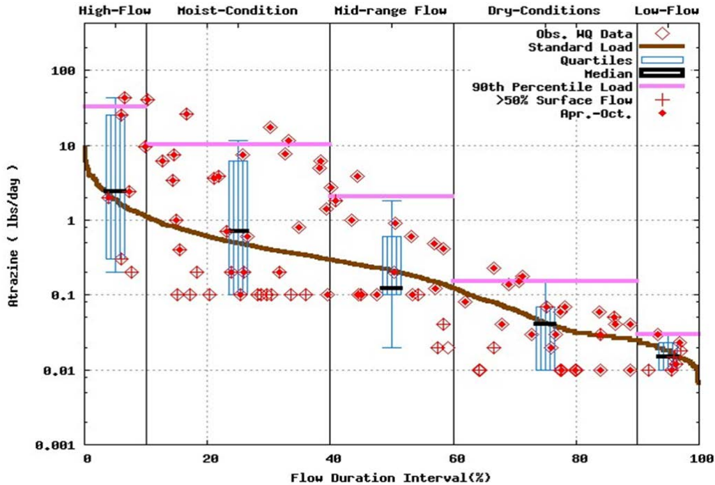
Figure 6. Load Duration Curve from Illinois EPA derived using flow data from USGS stream gage 0338780 and Syngenta provided data set for atrazine loadings to N. Fork Vermillion River.
