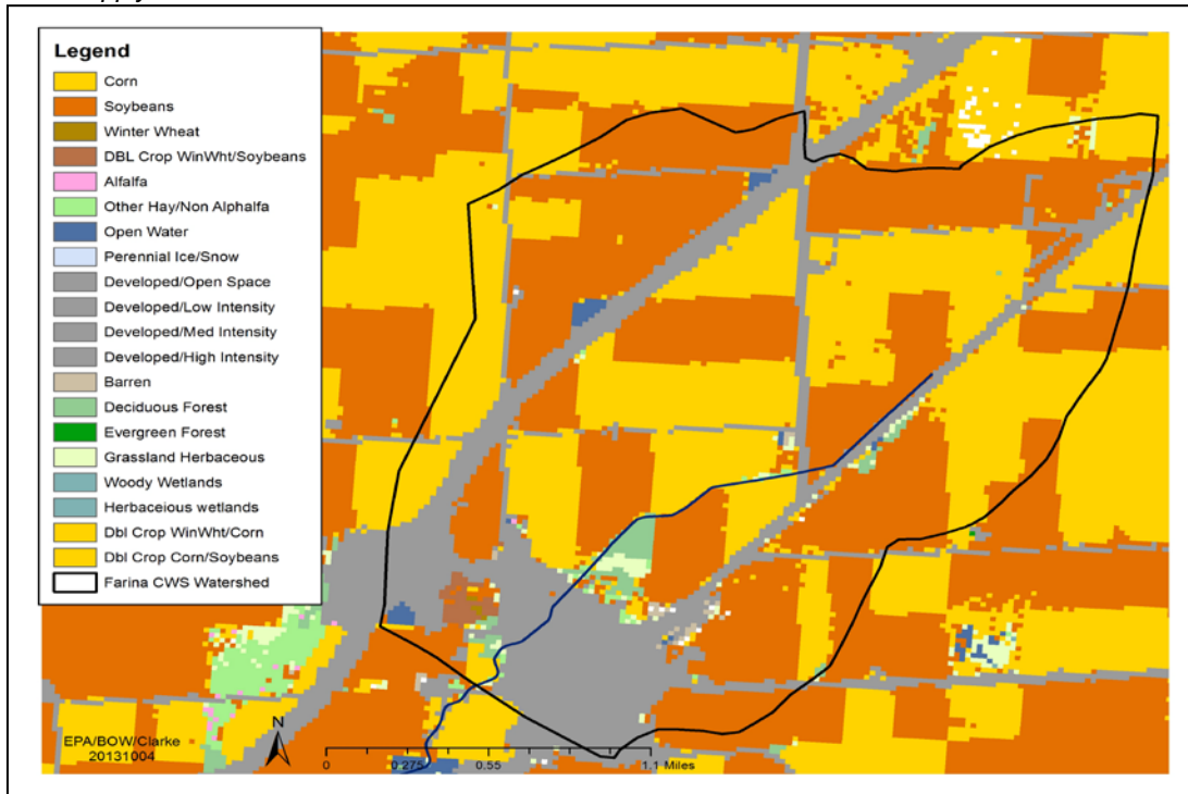
Figure 2. Landuse in the East Fork Kaskaskia River Watershed Upstream of the Farina Community Water Supply Intake
