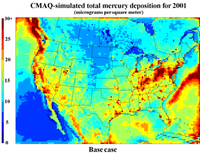
Figure 5.1 CMAQ – Simulated Mercury Deposition For 2001, Base Case
