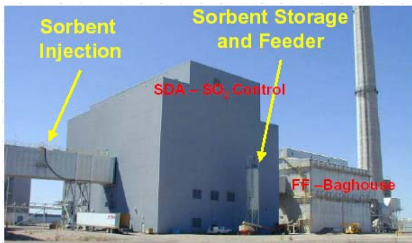
Figure 8.8 Sorbent Injection equipment compared to other air pollution control equipment (Durham, 2005).
