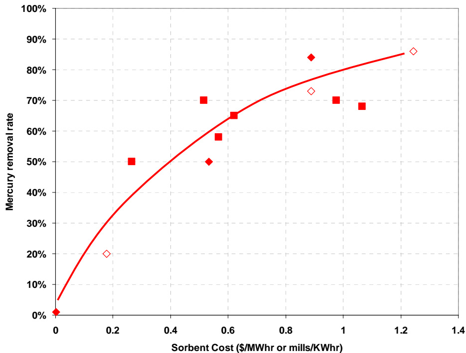
Figure 8.14 Estimated Cost Impact to Generation of Sorbent for Mercury Removal on a Bituminous Coal-Fired Boiler using Halogenated PAC
