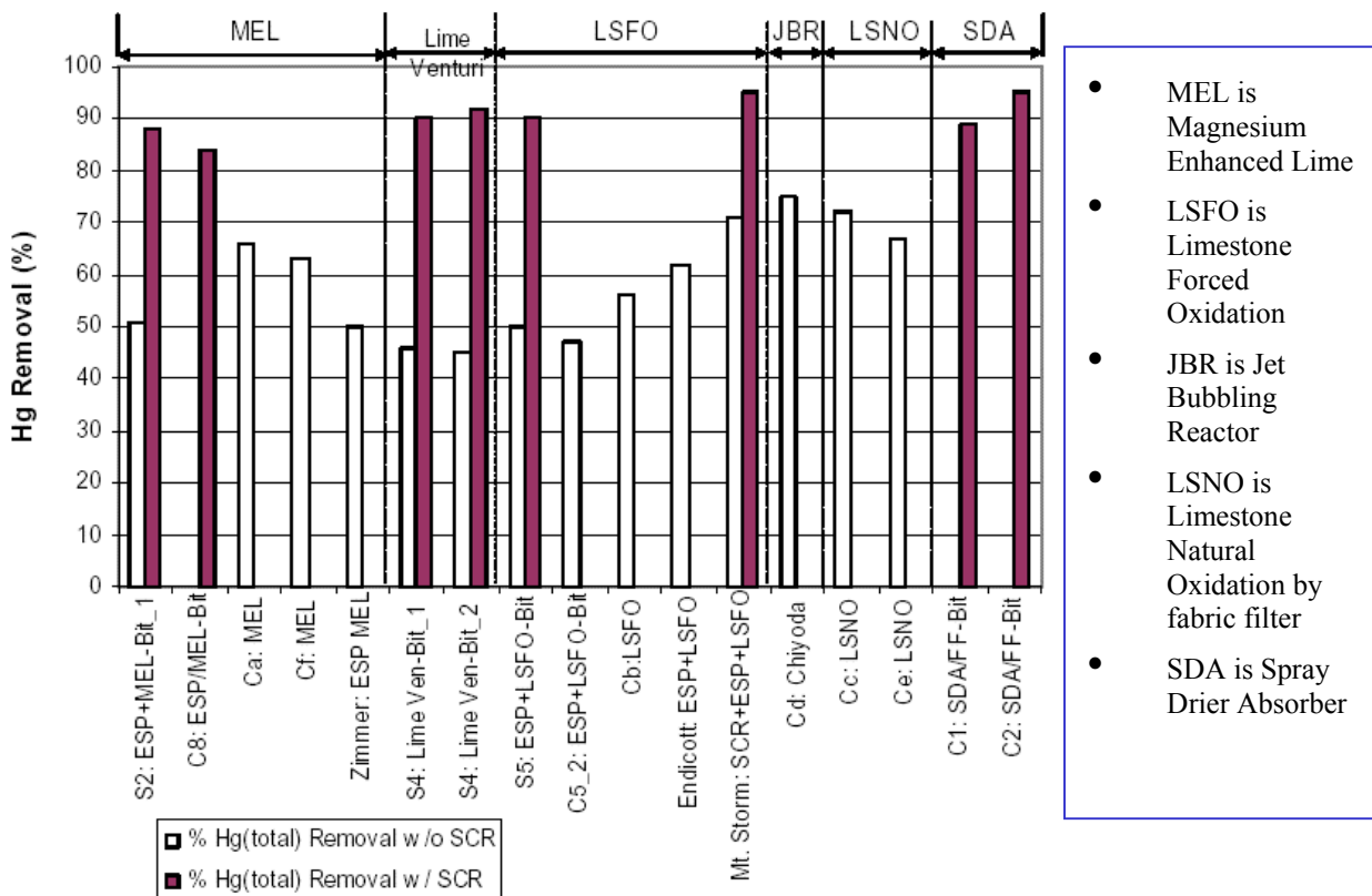
Figure 8.3. Mercury Removal by Wet FGD Technology With and Without SCR (USEPA, 2005)
